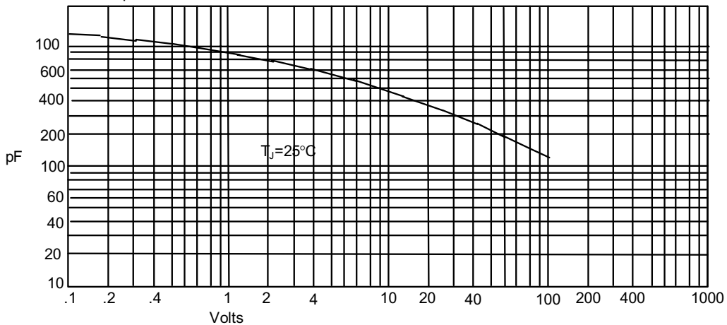
Figure 3 Junction Capacitance
