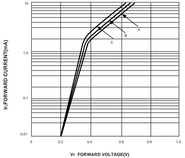
FIG. 2-TYPICAL FORWARD CHARACTERISTIC
