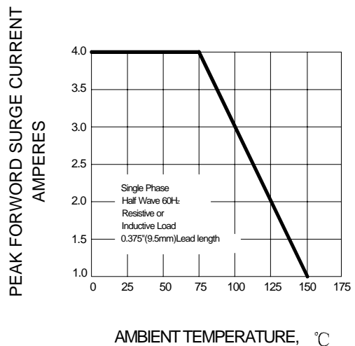
FIG.5-FORWARD DERATING CURVE
