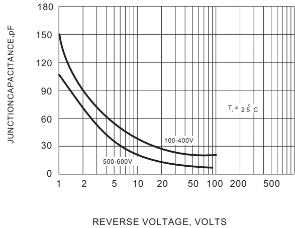
Fig.2 TYPICAL JUNCTION CAPACITANCES
